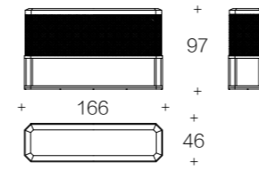
D-XXCG-01 | 餐边柜 1660*460*970
